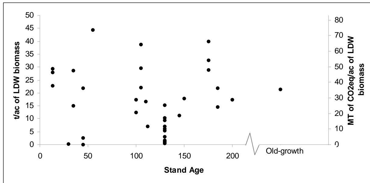
Figure 8 LDW quantities in Western interior coniferous forests
