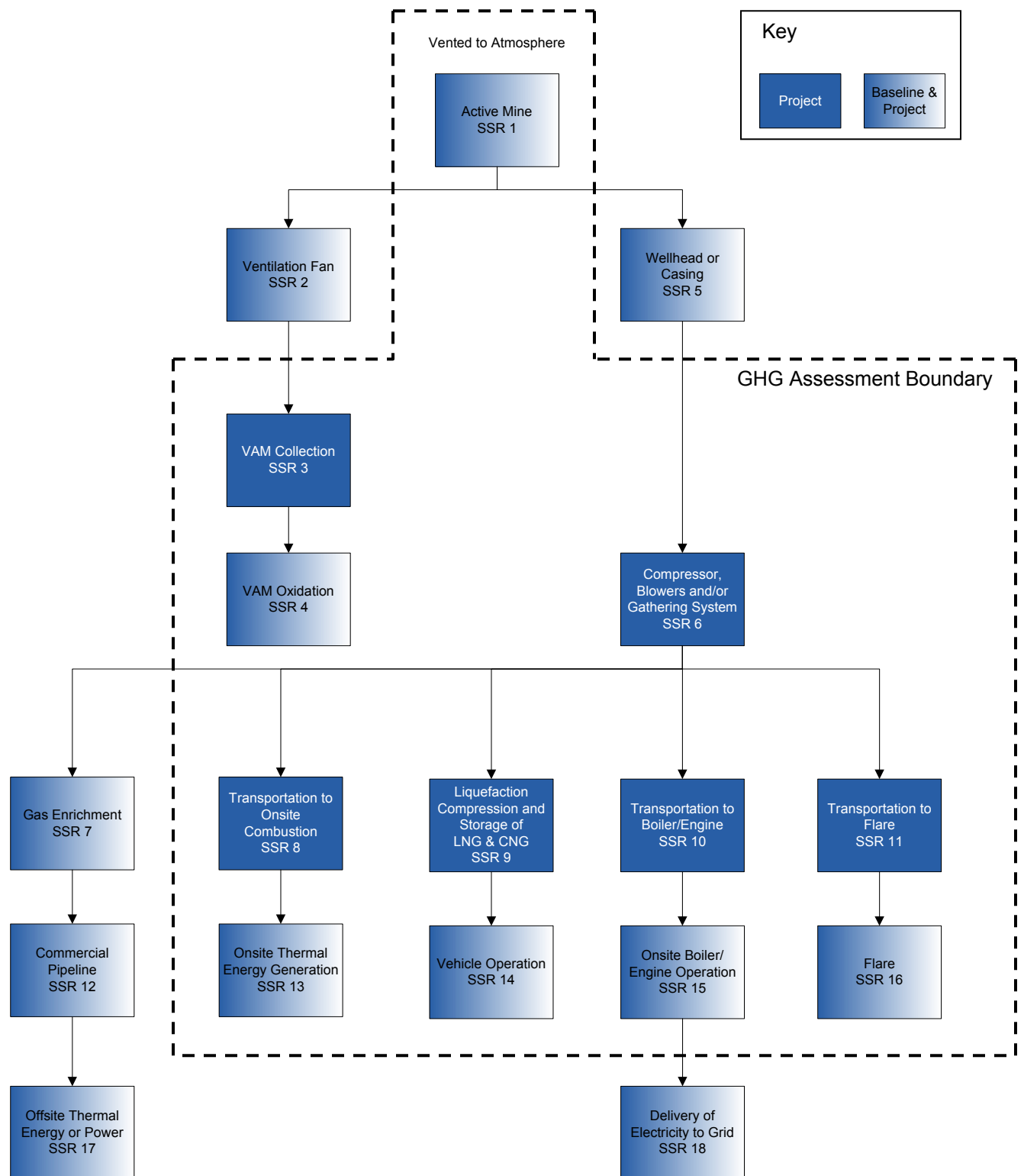
Figure 4.1. Illustration of the GHG Assessment Boundary
