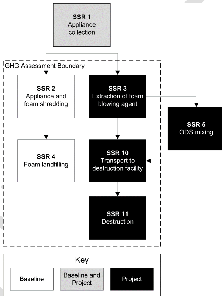
Figure 4.1. Reduction Project Process for ODS Contained in Foam
