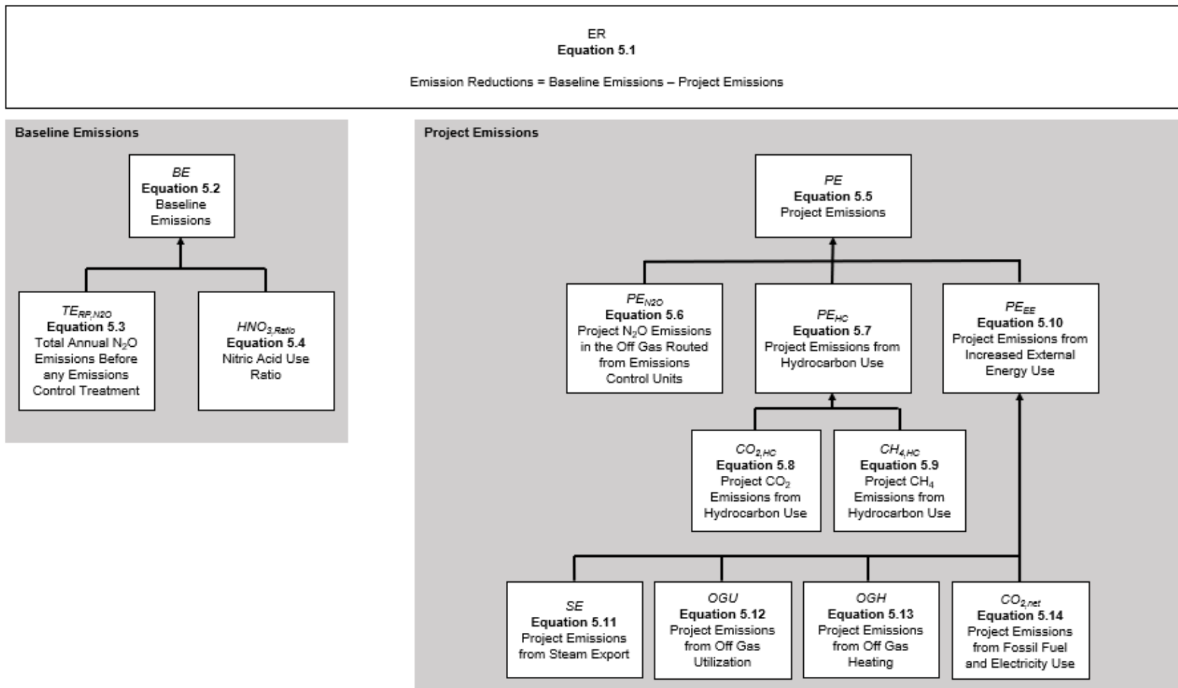
Figure 5.1. Organizational Chart of Equations for Adipic Acid Projects
